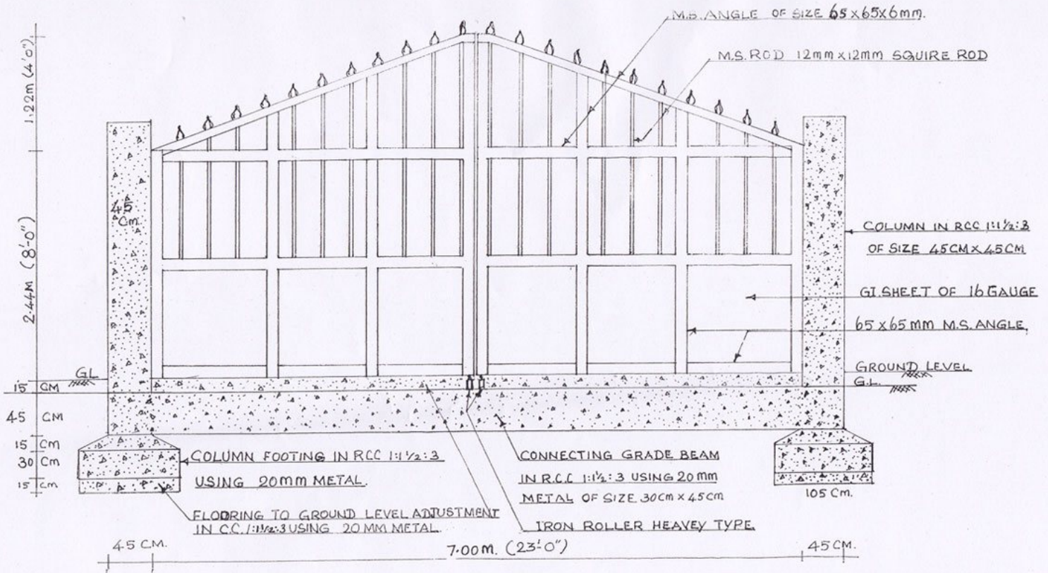
SKETCH SHOWING THE MAIN ENTRANCE GATE AT FOOT OF THE HILL OF A/M MANTHIRAGIRI VELAYUTHASWAI THIRUKOIL AT THENCHERIMALAI SULLUR, TALUK, TIRUPPUR DISTRICT SCALE 1CM=30CM
